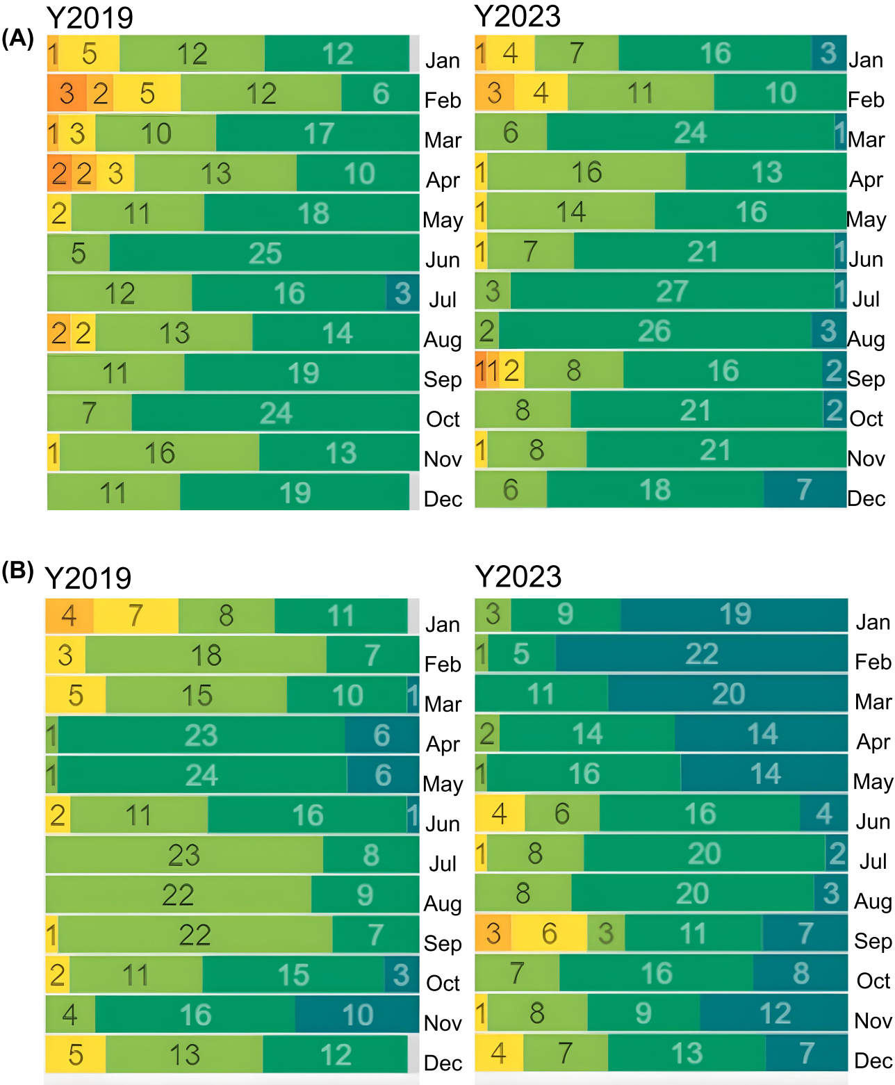
Fig. (4). Annual air quality measurement values in London (a) and Madrid (b) before and after COVID-19 [28].
